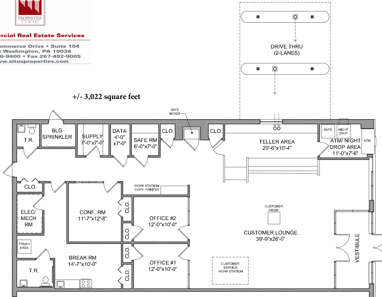
FLOOR PLAN SCALE: \frac{3}{32} " = 1'-0"
