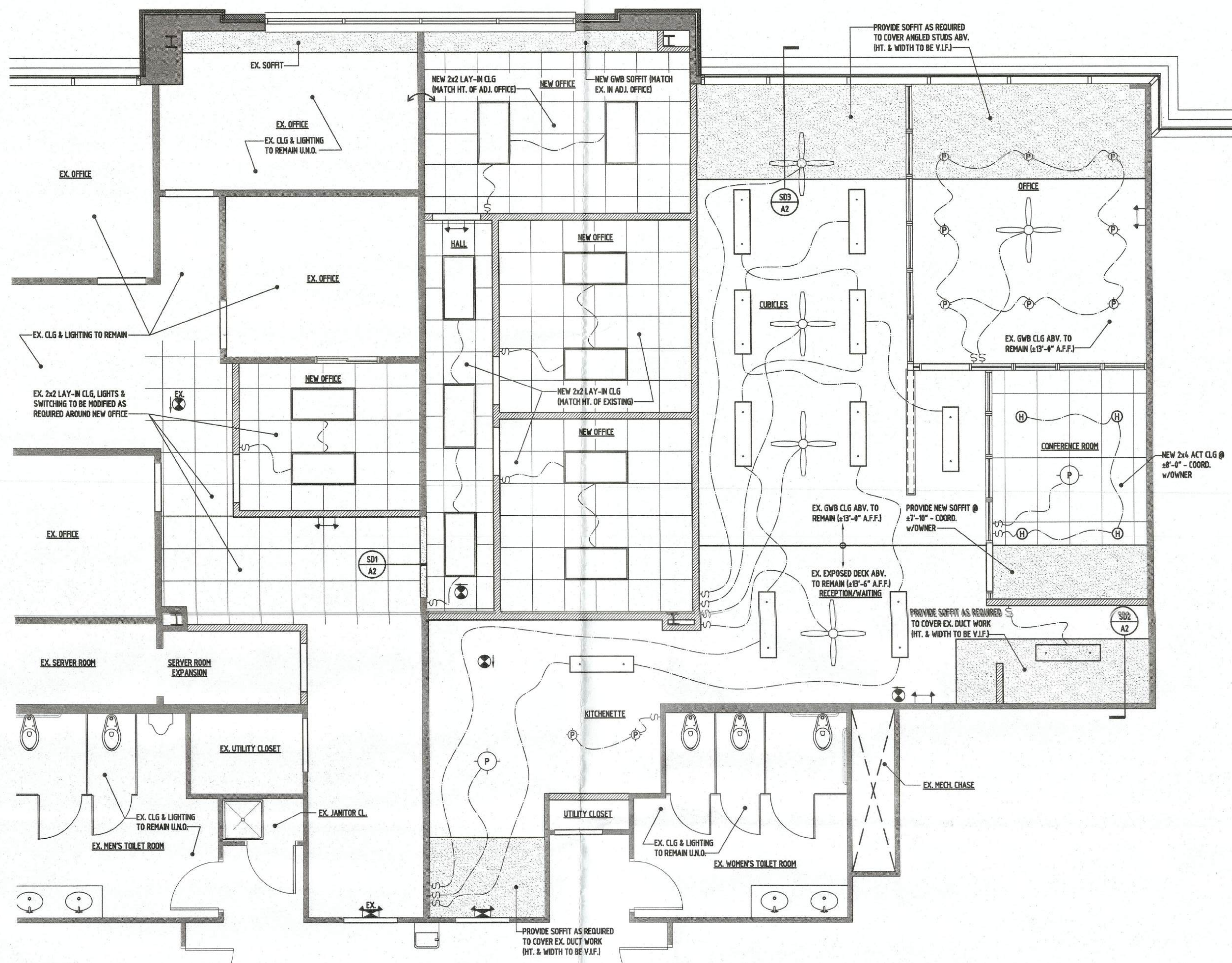
PARTIAL SECOND FLOOR REFLECTED CEILING PLAN
