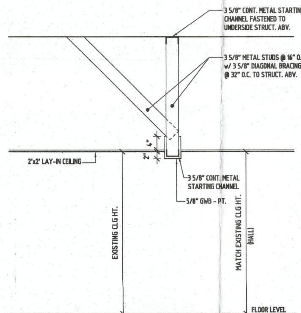
SD1 SOFFIT DETAIL
