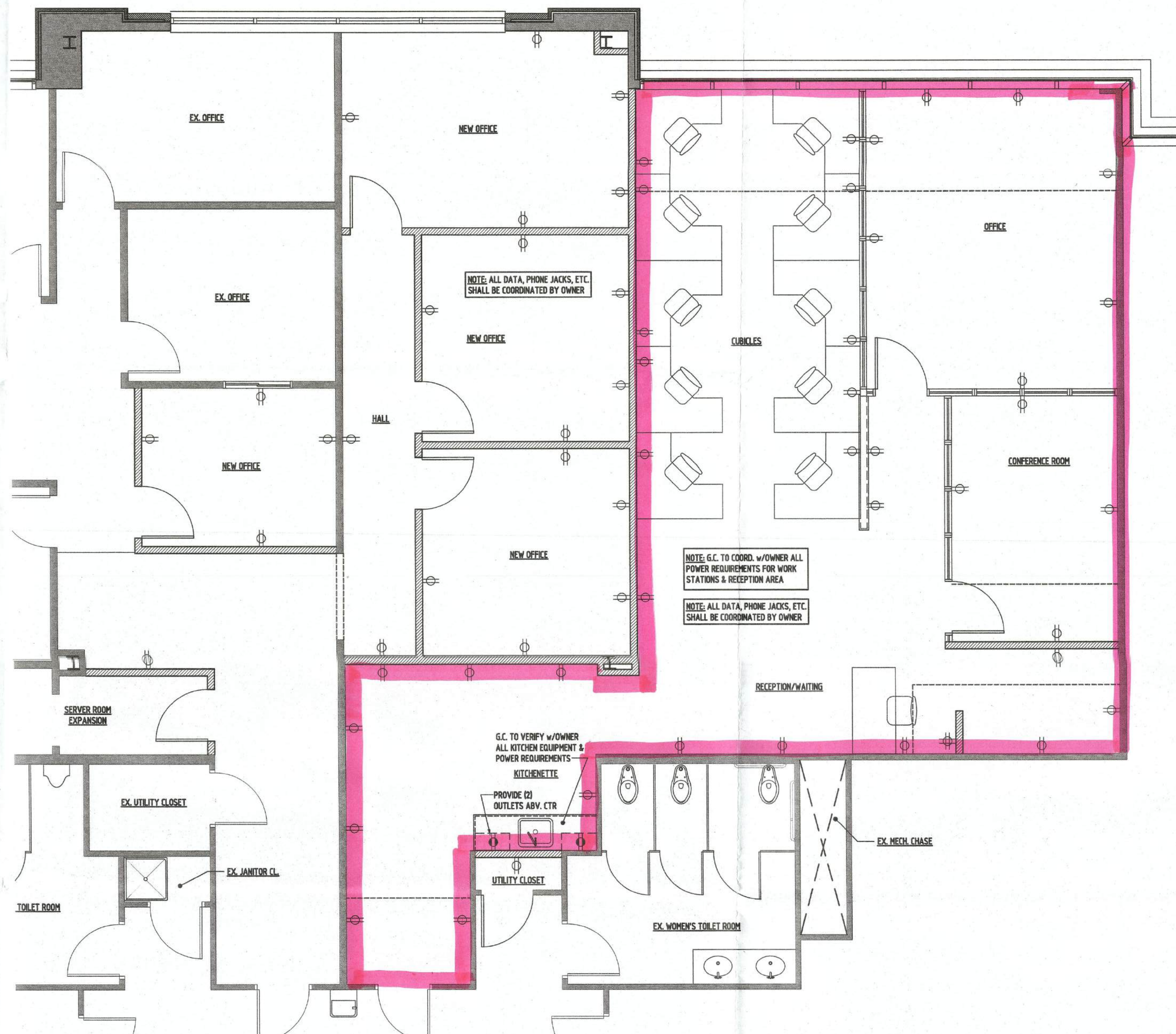
PARTIAL SECOND FLOOR ELECTRICAL PLAN
