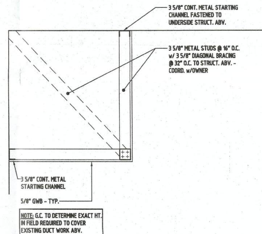
SD2 SOFFIT DETAIL
