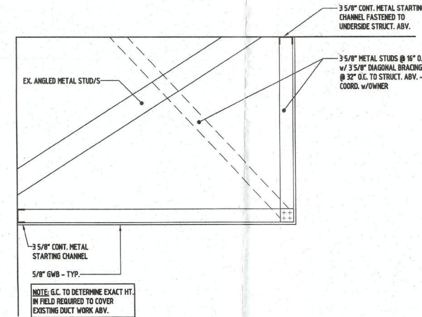
SD3 SOFFIT DETAIL
