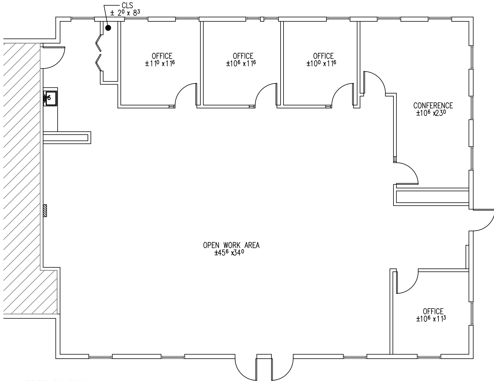
EXISTING FLOOR PLAN SCALE: 1/8" = 1'-0"
