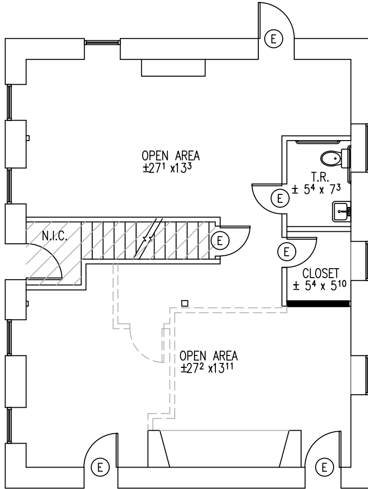
SK.1 FIRST LEVEL PLAN SCALE: 1/8" = 1'-0"
