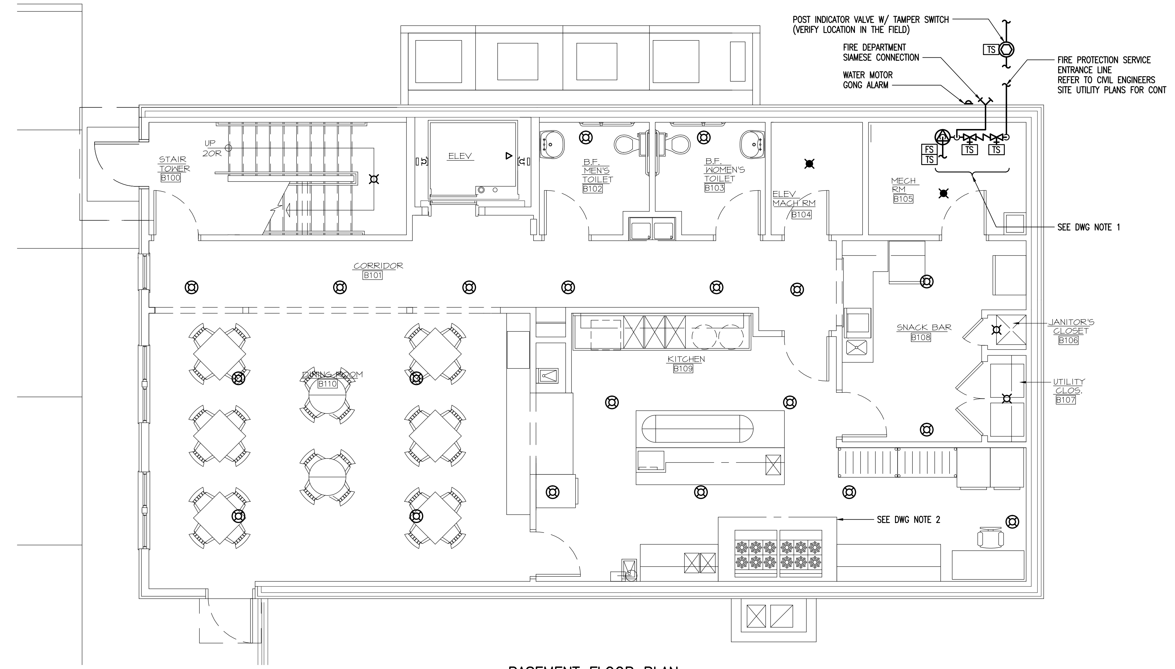
BASEMENT FLOOR PLAN SCALE: 1/4" = 1'-0" (FN FLR EL 106.34')
